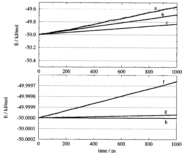
FIG. 10. Evolution of total energy for the three lowest (top) and highest (bottom) accuracies in Fig. 9 for a quaternion/extrapolation integration scheme. All curves are smooth but drift away from the initial energy.
